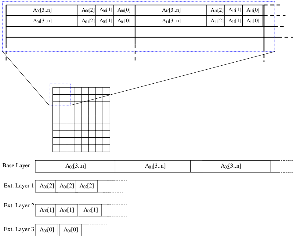
Figure 6: MPEG spatial resolution layers. MPEG transforms 8x8 blocks of pixels into 8x8 blocks of coefficients from the 2-dimensional discrete-cosine transform (DCT). Each coefficient is denoted A_{ij} , and the bits of an individual coefficient are indexed A_{ij}[0..n] . Quantization, dropping low-order bits, is the main lossy component of the MPEG compression technique, resulting in loss of spatial detail. In MPEG transcoding, the low-order bits of each MPEG coefficient are progressively assigned to layers starting from the highest extension layer and ending with the lowest, with the base layer containing all remaining bits. Eliminating MPEG layers corresponds to increasing quantization in the MPEG encoding process.
