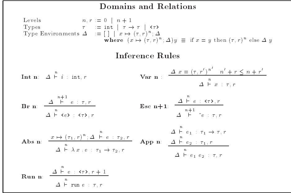
Fig. 1. Type System
